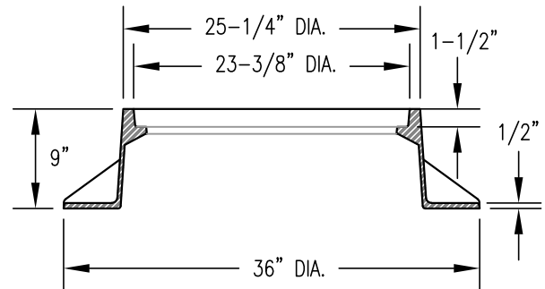
NEENAH CASTING R-1916-C PRODUCT # 1916-0281 COMPLETE ASSEMBLY:1916-315
