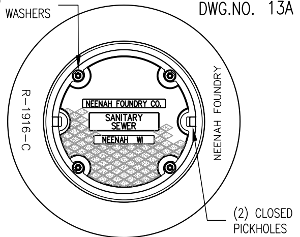
NEENAH LID: 1916-0339 NON-VENTED/NON-GASKETED
