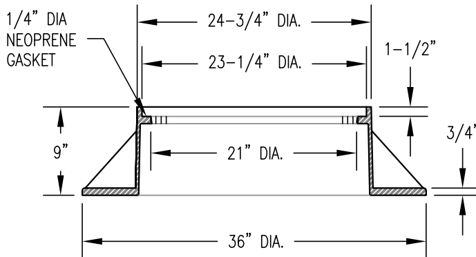
EJ CASTING NO. 1058ZPT PRODUCT # 00105812 COMPLETE ASSEMBLY:1058ZPT/APT PRODUCT # 00105807
