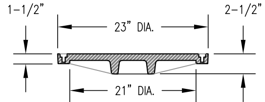
NEENAH LID: 1916-0339 NON-VENTED/NON-GASKETED
