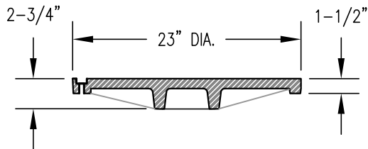
EJ LID: 1058APT PRODUCT # 00105826
